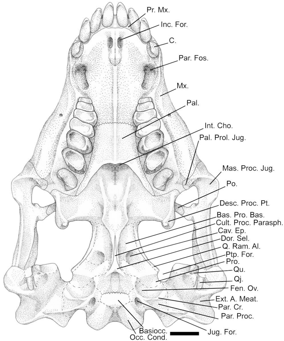
TEXT-FIG. 5. Illustration (with reconstructions) of the Skull of Protuberum cabralensis in palatal view. Bas. Pro. Bas., basiptyergoid process of the basisphenoid, Basiocc., basioccipital, C., canine, Cav. Ep., cavum epiptericum, Cult. Proc. Parasph., cultriform process of the parasphenoid, Desc. Proc. Pt., descending process of the pterygoids, Dor. Sel., dorsum sellae, Ext. A. Meat., external auditory meatus, Fen. Ov., fenestra ovalis, Int. Cho., internal choanae, Inc. For., incisive foramina, Jug. For., jugular foramen, Mas. Proc. Jug., masseteric processes of the jugals, Mx., maxilla, Occ. Cond., occipital condyle, Pal. Palatine, Pal. Prol. Jug., palatine prolongation of the jugal, Par. Cr., parotic crest, Par. Fos., paracanine fossa, Par. Proc., paroccipital process, Po., postorbital, Pro., prootic, Ptp. For., pterygoparoccipital foramen, Pr. Mx., pre-maxilla, Qj., quadratojugal, Q. Ram. Al.,
